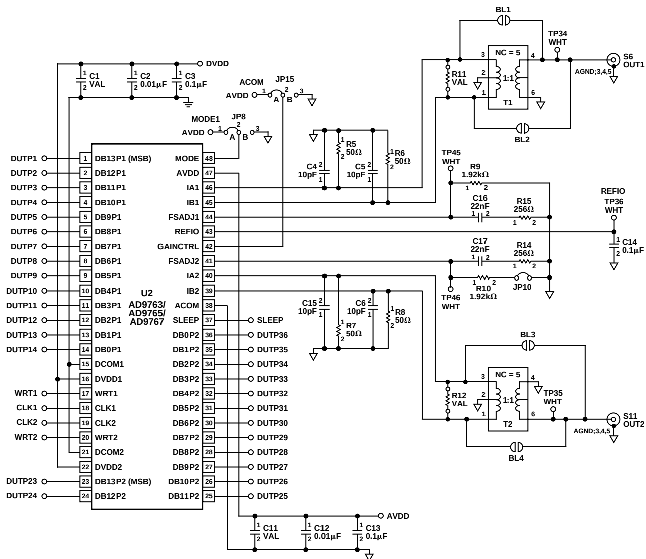
DUT AND ANALOG OUTPUT SIGNAL CONDITIONING
